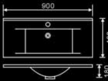
DB-9090D DB-9090D Size: 900x460x180 mm DB-9080D Size: 800x460x180 mm
