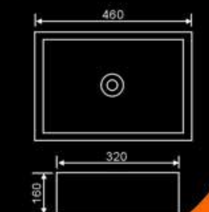
DB-7238 Size: 460x320x160 mm
