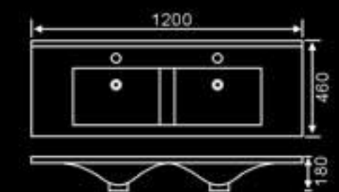
DB-9120ED Size: 1200x460x180mm
