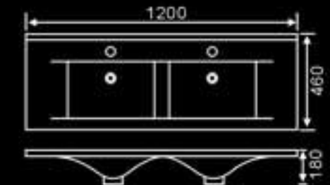
DB-9120DD Size: 1200x460x180 mm
