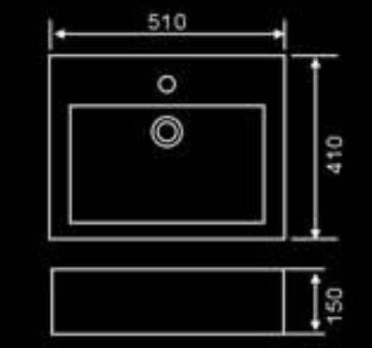
DB-7033 Size: 510x410x150 mm
