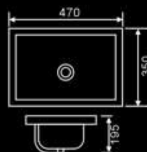
DB-540N Size: 470x350x195 mm DB-540F Size: 510x380x175mm
