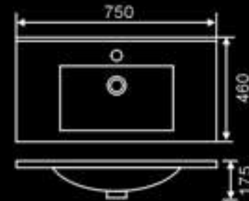
DB-9075E DB-9075E Size: 750x460x175mm DB-9070E Size: 700x460x175 mm DB-9080E Size: 800x460x175 mm
