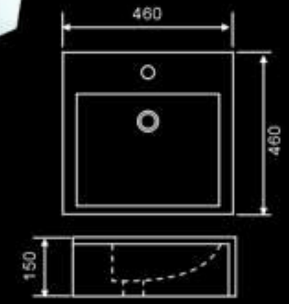
DB-7029AB Size: 460x460x150 mm
