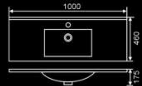
DB-9100E Size: 1000x460x175 mm
