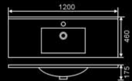
DB-9120E Size: 1200x460x175 mm
