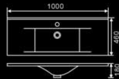
DB-9100D Size: 1000x460x180 mm
