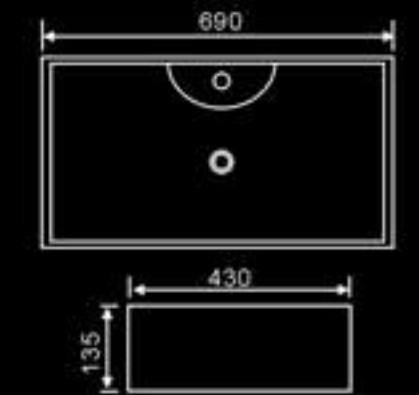
DB-7235B Size: 690x430x135 mm
